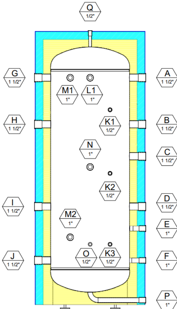
GSE CASCADE BF VER-FW-CF 300 INOX/LR
